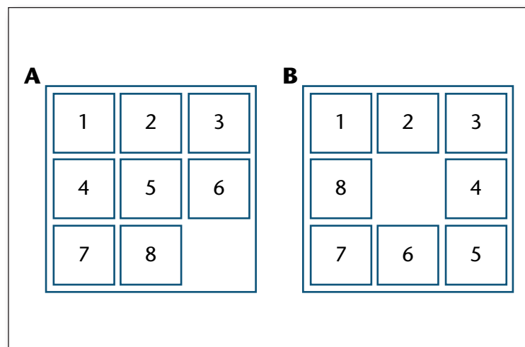
Figure 1. Goal Configurations of the 8-Puzzle.
