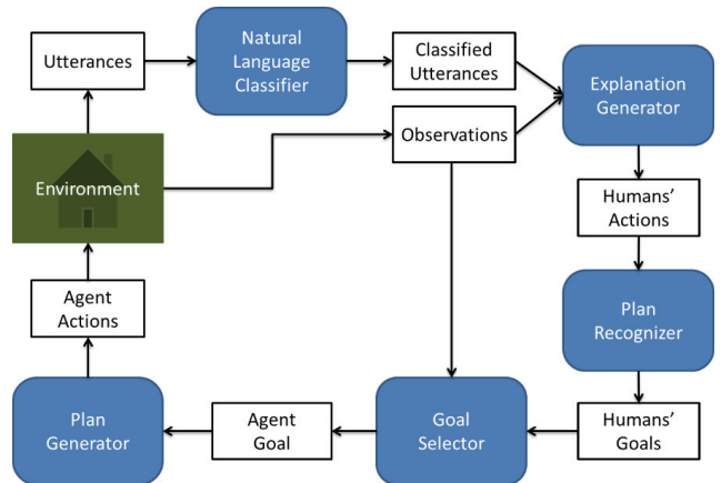
Figure 1: Decision cycle of the goal reasoning agent
