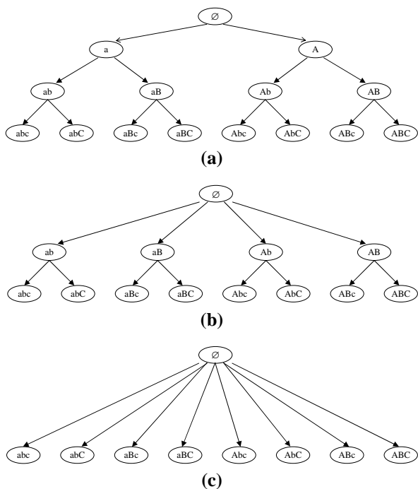
Figure 1: Search trees for a three-binary-variable MAP problem (a) full search tree instantiate one variable at a time, (b) search tree utilizing two-variable joint heuristic, (c) search tree utilizing three-variable joint heuristic.
