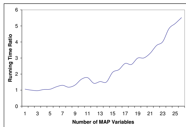
Figure 3: Ratio of the running time of DFBnB using individual bounds to the running time of DFBnB using joint bounds in solving the MAP problem for the Munin4 network, as a function of the number of MAP/evidence variables.
