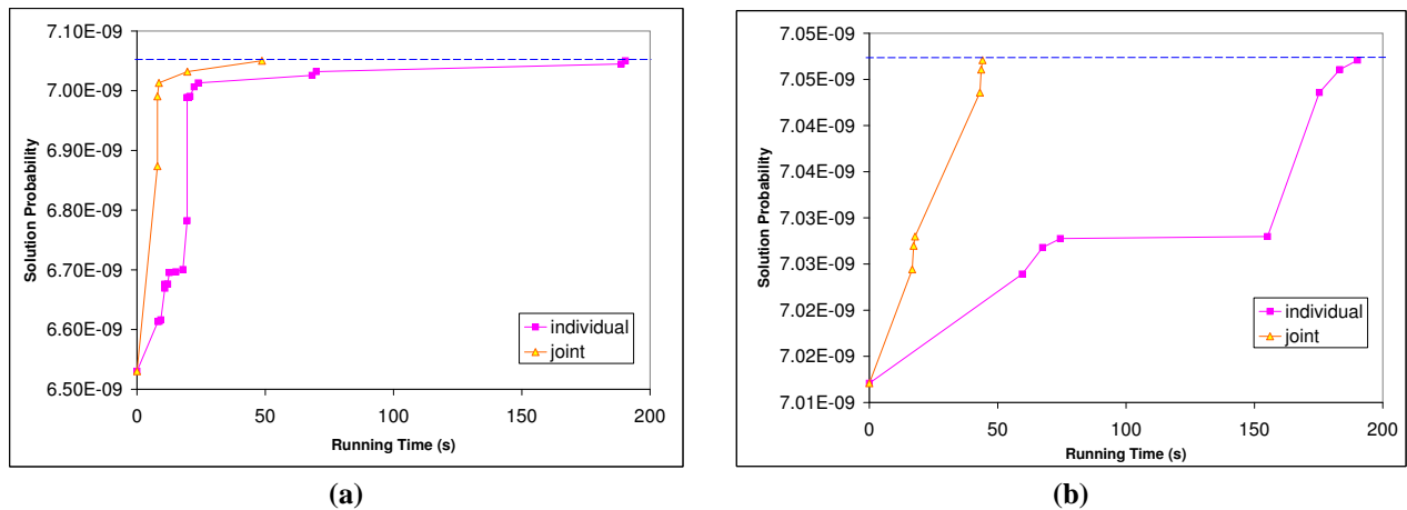
Figure 2: Comparison of DFBnB using individual and joint bounds in finding the best solution for two test cases of the Mildew network. (The horizontal line shows the best solution found.)
