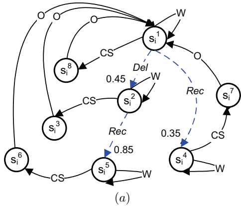
Figure 3: (a) A (probabilistic) state transition diagram illustrating the expanded transition function, T_i^E , for the SM i . Transitions due to actions are depicted using solid lines, and these are deterministic. Exogenous events are shown dashed. For clarity, the occurrence of no event is not shown. The numbers denote example probabilities of occurrence of the events conditioned on the states. (b) The partial cost function for the PM. We show the costs for the more interesting actions of waiting and changing the supplier, for a subset of the states. The cost function penalizes those action combinations where only one SM changes the supplier thus violating the compatibility constraint.
