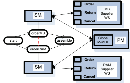
Figure 2: The PM does the global decision making for adaptation using the M-MDP model.
