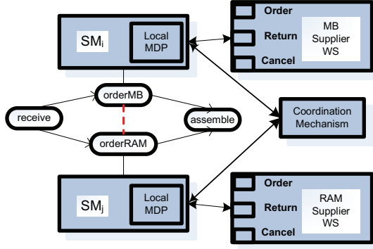
Figure 6: Each SM locally decides its action in response to the events. The SMs coordinate using a CoM that each observes perfectly.
