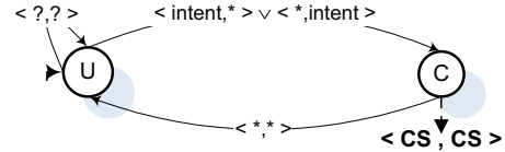
Figure 7: FSM for coordinating between the SMs. Transitions (solid arrows) are caused by the joint actions of the SMs. '*' indicates any action of a SM, while '?' indicates the remaining actions. The dashed arrow gives the action rule for each SM when the FSM is in that state.
