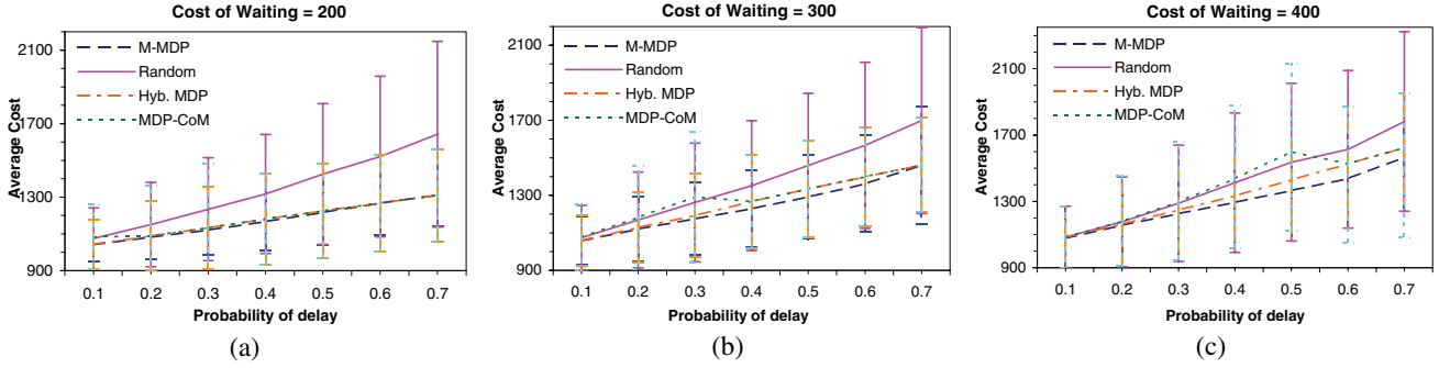
Figure 10: Line plots showing the average costs incurred for increasing probabilities of the order being delayed and increasing costs of waiting for the order in response to the delay. The vertical lines in each plot show the standard deviations.
