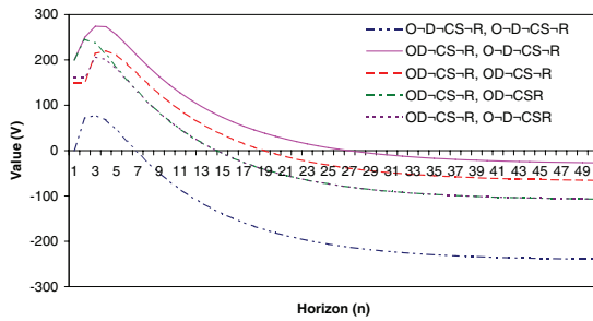
Figure 9: Convergence of the value function of the M-MDP model.
