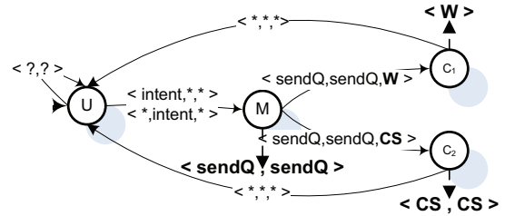
Figure 8: The CoM for our hybrid approach.
