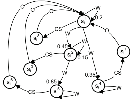
Figure 4: A (probabilistic) state transition diagram illustrating the transition function, T_i , for the SM i . Some of the transitions due to the actions are now non-deterministic. The numbers denote the probabilities with which the associated transitions occur.
