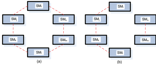
Figure 5: Example coordination graphs. (a) The worst case coordination graph where all the SMs must coordinate with each other. (b) More realistic case, where only subsets of SMs must coordinate.
