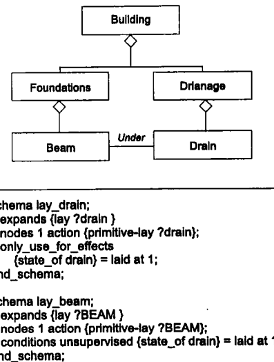
Figure 10: Dependency Encoding Example, Different Parentage Case
