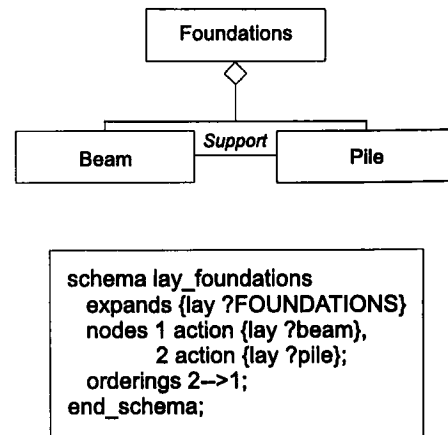
Figure 9: Dependency Encoding Example, Same Parentage Case
