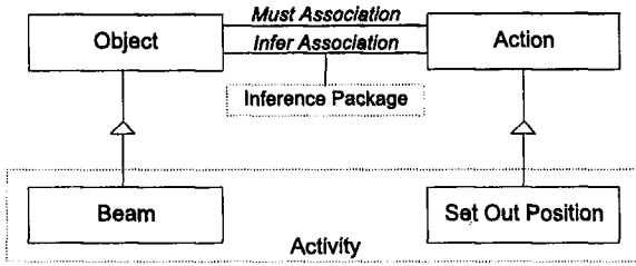
Figure 1: An Activity Defined as the Union of an Object and an Action
