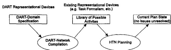
Figure 11: DART-Network Architecture
