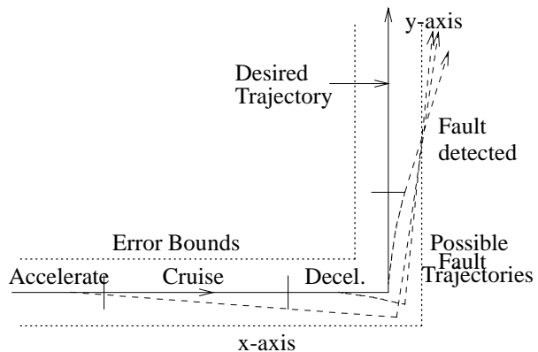
Figure 1: Trajectories of AERCam under various possible faults. The fault trajectories are simplified for illustration purposes.
