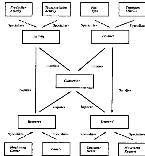
Figure 2: Layered models of scheduling subdomains
