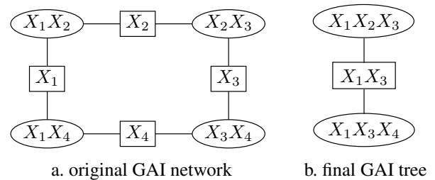
Figure 6: A GAI tree resulting from a triangulation.
