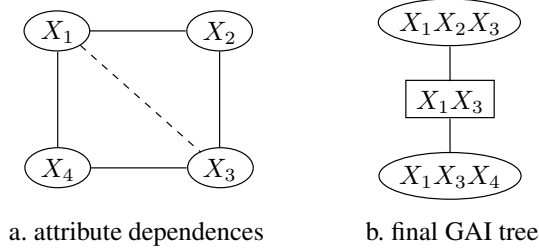
Figure 4: From a GAI network to a GAI tree.
