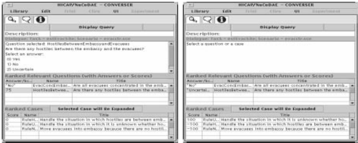
Figure 4: NaCoDAE/HTN’s interface, before (left) and after (right) answering a question. The top window directs the user and lists the possible answers. The lower windows display the questions and cases, respectively.
