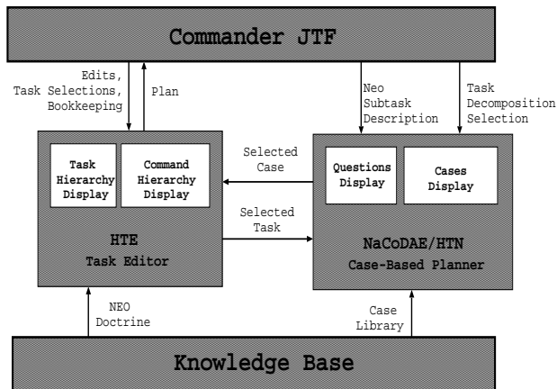
Figure 1: The HICAP architecture.
