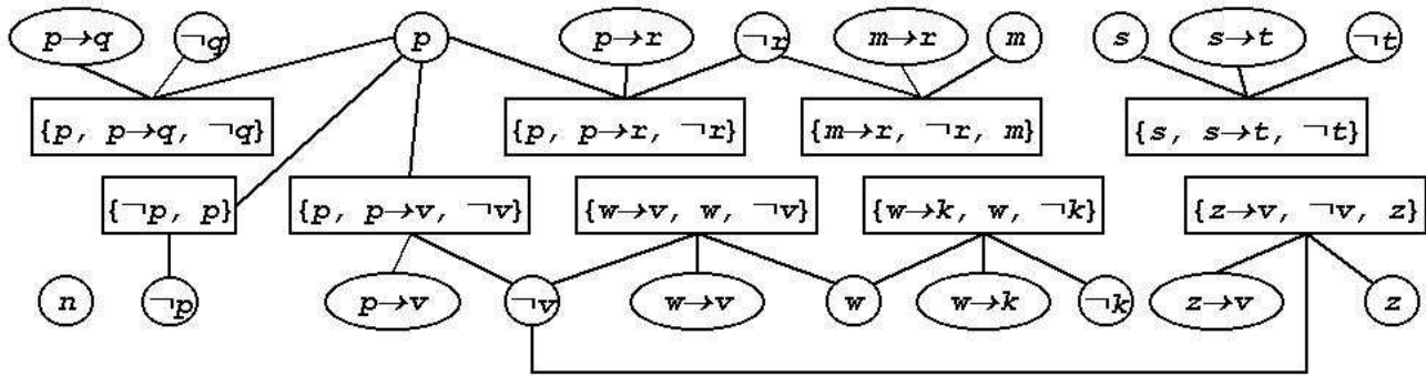
Figure 1: A graph showing the elements of B^U (circles/ovals) of a KS connected to their inconsistent sets (rectangles). If \neg p was not yet added to the base, and we had an IAT-preference ordering that ordered the beliefs in the following sequence from most to least preferred: p, p \rightarrow q, p \rightarrow r, m \rightarrow r, s \rightarrow t, w \rightarrow v, w \rightarrow k, p \rightarrow v, z \rightarrow v, n, \neg r, w, s, \neg v, m, z, \neg q, \neg t, \neg k , then the optimal base would be B1 = \{p, p \rightarrow q, p \rightarrow r, m \rightarrow r, s \rightarrow t, w \rightarrow v, w \rightarrow k, p \rightarrow v, z \rightarrow v, n, w, s, m, z\} . The semi-revision addition of \neg p (preferred over p ) followed by reconsideration is described in Example2.
