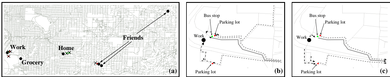
Figure 3: (a) Street map along with goals (dots) learned from 30 days of data. Learned trip switching locations are indicated by cross marks. From home, the person either walks to one of the two bus stops or takes the car, which is not learned as a trip switching location since the car is parked inside the house. (b) Zoom into the area around the work place. Shown are very likely transitions (probability above 0.75), given that the goal is the work place (dashed lines indicate car mode, solid lines bus, and dashed-dotted lines foot). (c) Learned transitions in the same area conditioned on the home being the goal.
