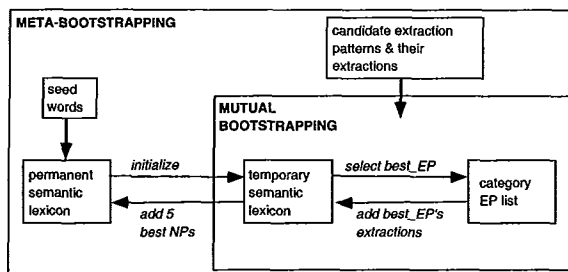
Figure 3: The Meta-Bootstrapping Process
