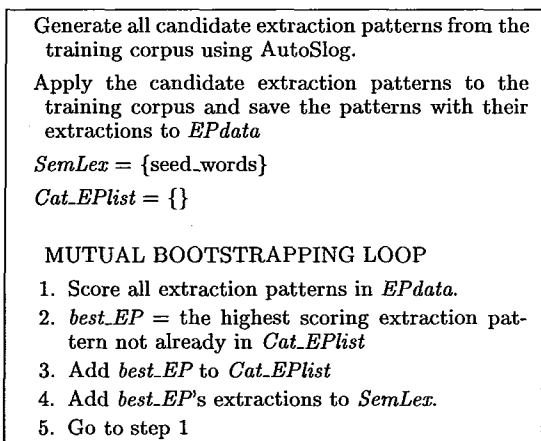
Figure 1: Mutual Bootstrapping Algorithm
