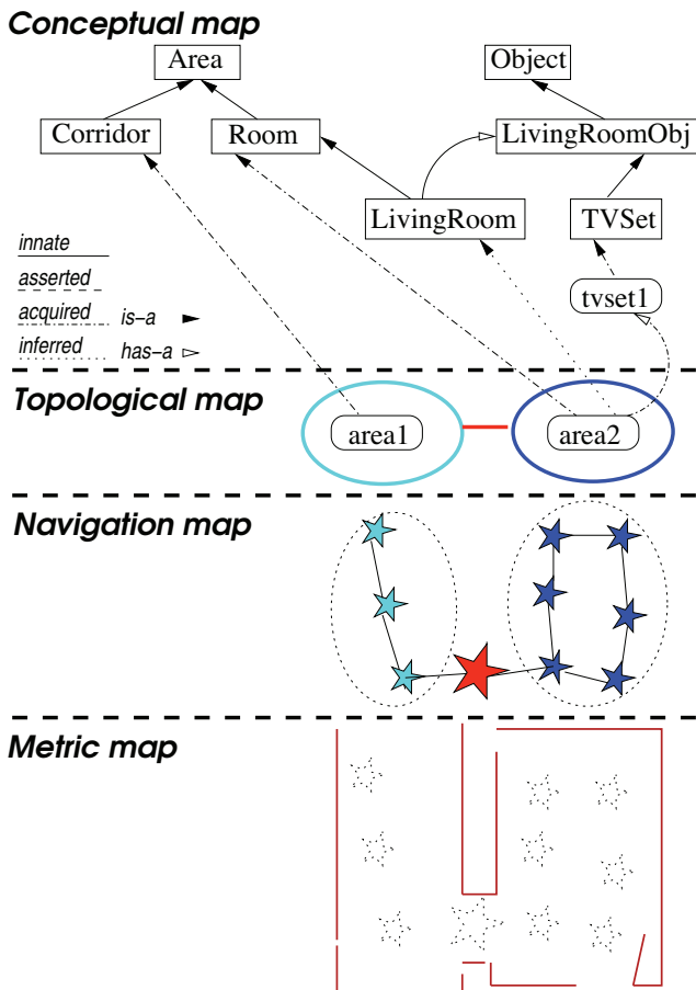
Figure 2: Multi-layered representation
