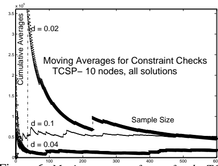
Figure 6: Moving averages for CC for the TCSP.
